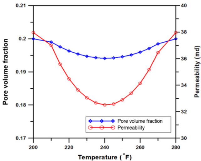
Fig. 12. Change of pore volume fraction and permeability due to asphaltene precipitation as a function of temperature (2,280 psi).
