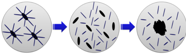
Fig. 1. Mechanism of asphaltene precipitation due to increasing temperature.
