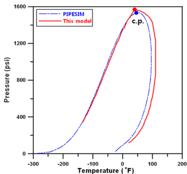
Fig. 3. Comparison of the phase envelope for light oil.
